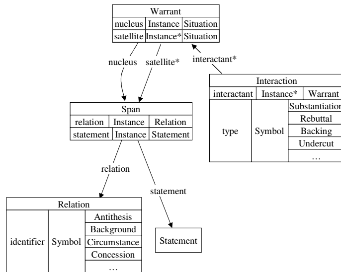
Fig. 1. DBR Reasoning Model
