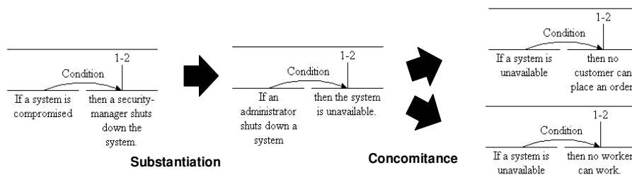
Fig. 2. Examples of Interaction Strategies
