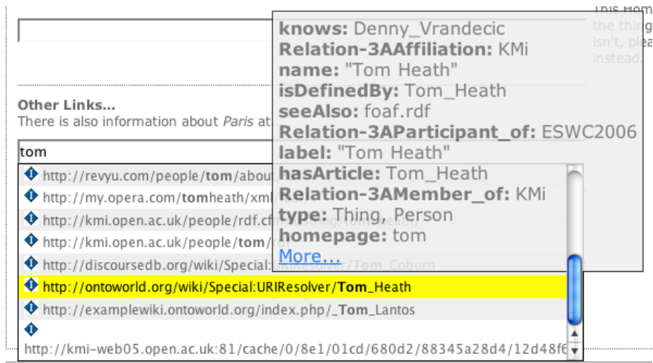
Fig. 1. MOAW suggesting URIs for “tom” on the Revyu.com website.
