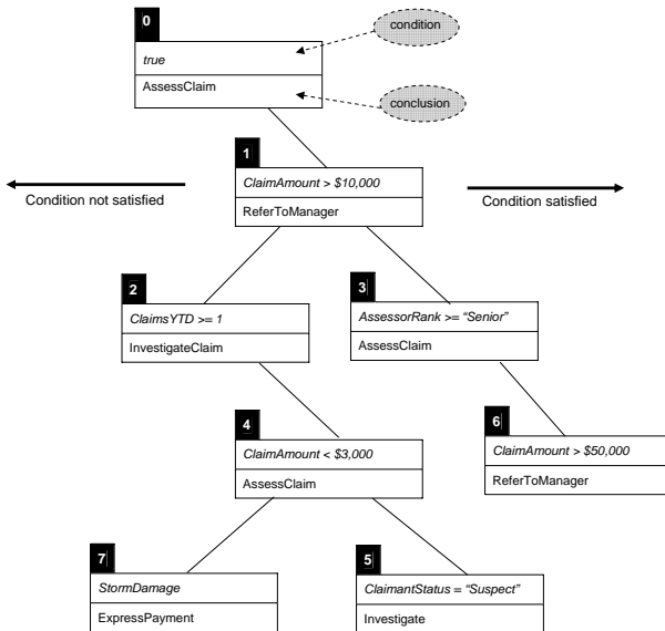
Fig. 1. Conceptual Structure of a Ripple Down Rule ( Assess Claim Example)
